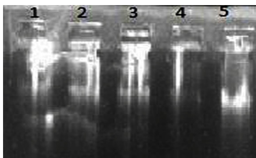
Figure 2. Agarose gel electrophoresis gel images of methanol extract of V. tmoleum . Ingredients of lines: Lane1: CT-DNA (3 mg/mL) in buffer (Tris HCl, pH=7), Lanes 2-5: CT-DNA (3-0.375 mg/mL) + buffer+ V. tmoleum (50 \mu M)
